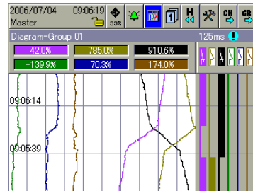
Recorder chart presentation of analog and binary channels
